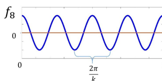
FIGURE 0.1. The 8th eigenfunction and its corresponding wave length.
